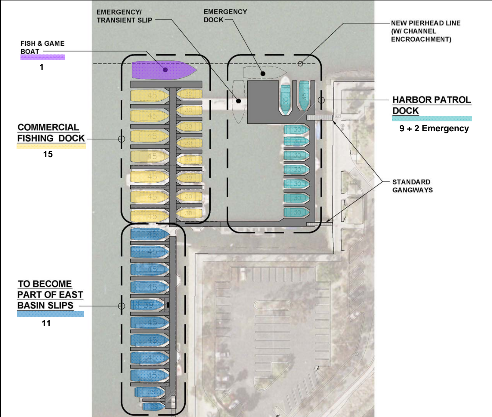
HARBOR PATROL / COMMERCIAL FISHING DOCKS CONCEPT
